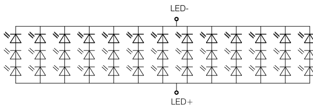
Backlight Circuit Diagram (LED 3*13=39 SMD) Color: WHITE
