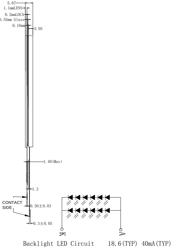
Backlight LED Circuit 18.6(TYP) 40mA(TYP)
