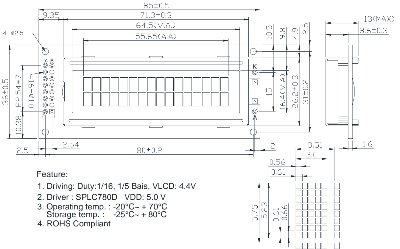
DOTS DETAIL SCALE=4:1
